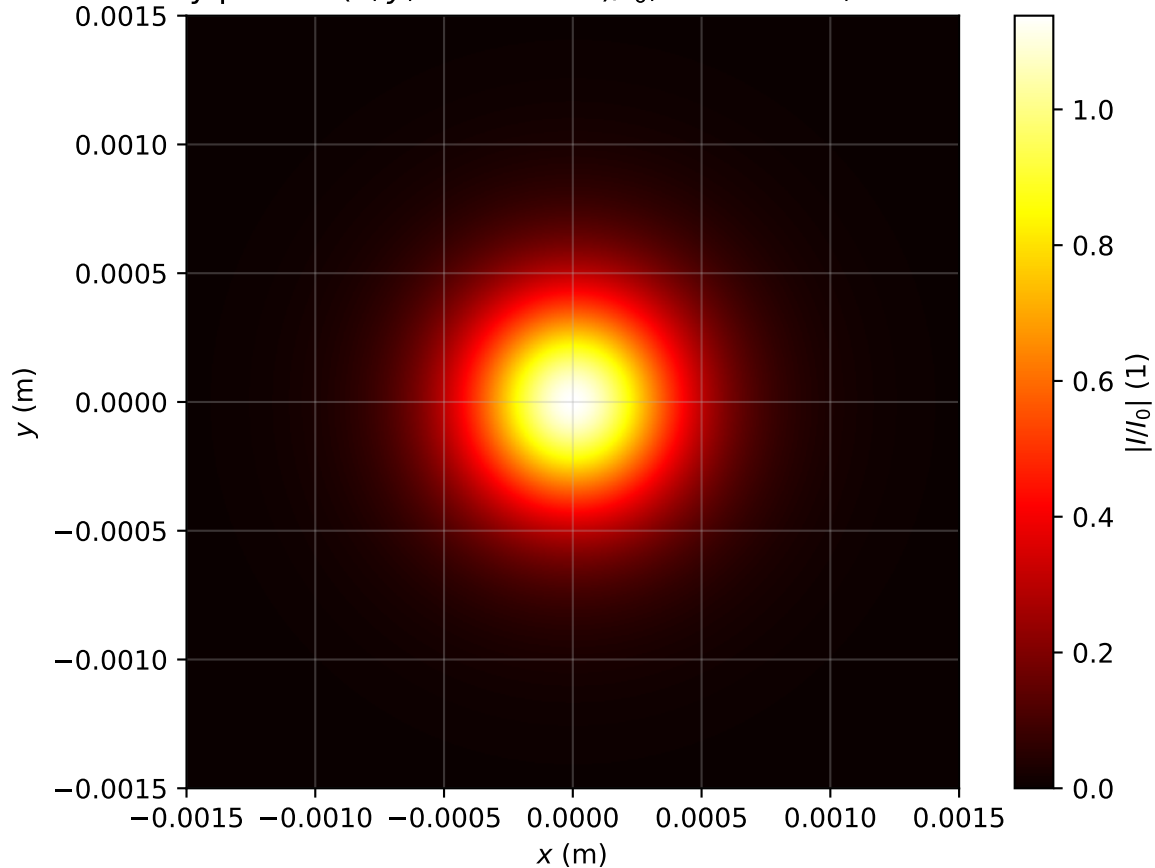
Intensity profile I(x, y, z = 1.831m)/I_0 , P_{in}=0.7P_{cr} , artificial time
